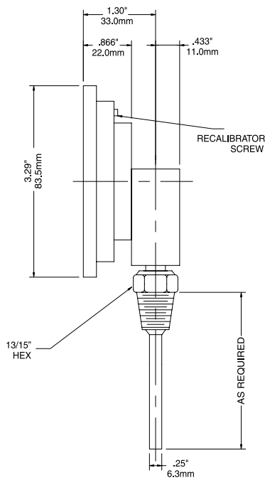
3" Bottom Connection
